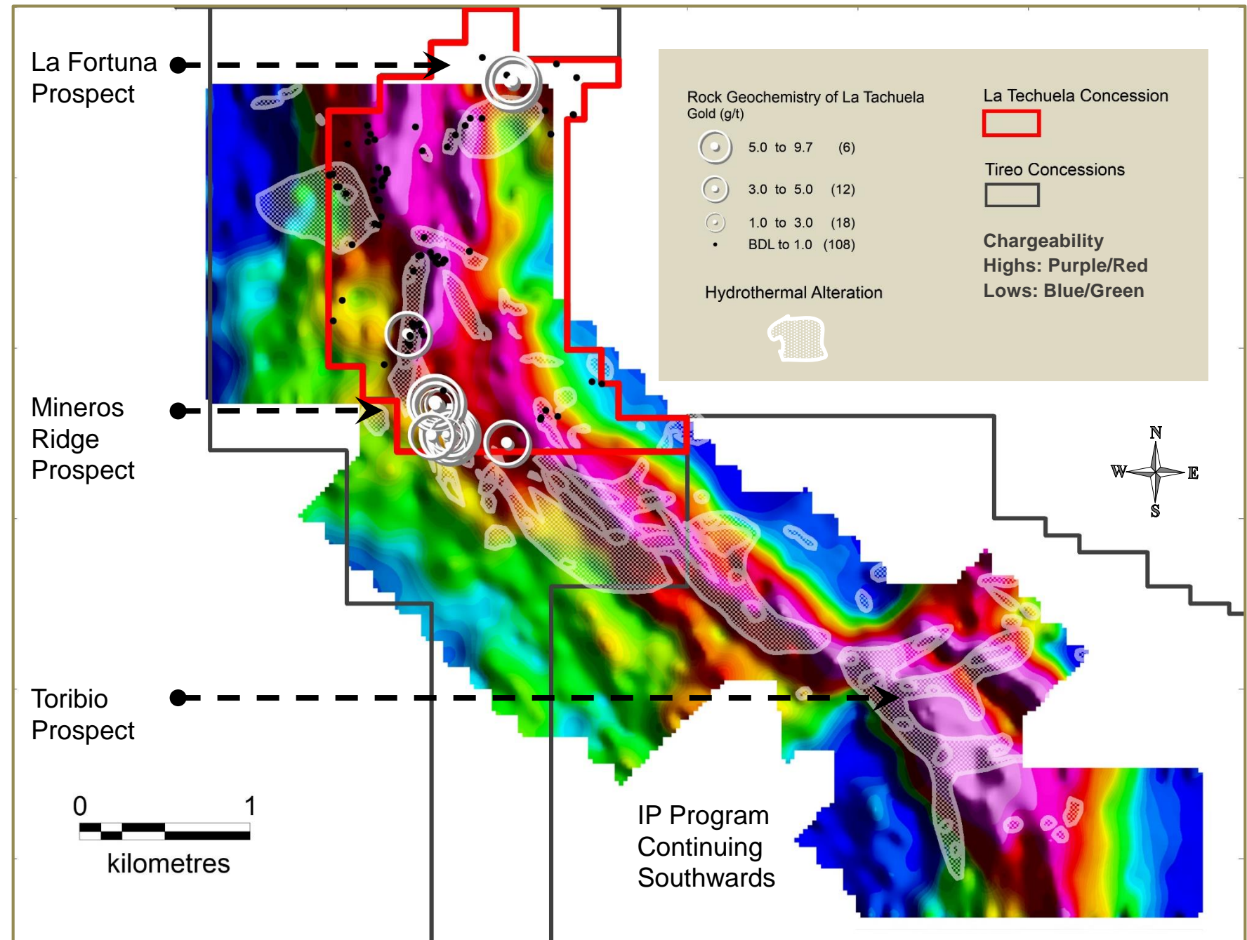
Fig 2: Updated 2016 IP Chargeability highlighting La Tachuela Concession
