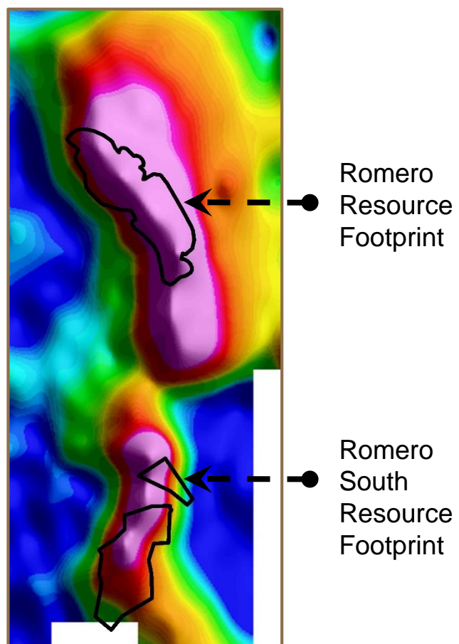
Fig 1: Romero Chargeability Anomaly (same scale)
